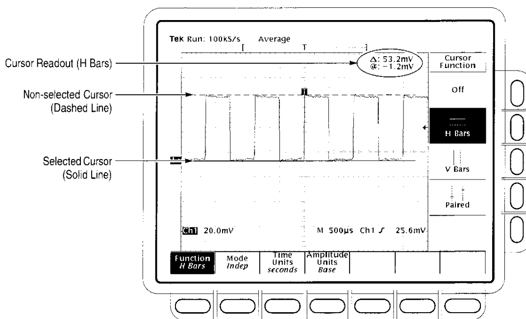
Figure 3–67: H Bars Cursor Menu and Readouts
