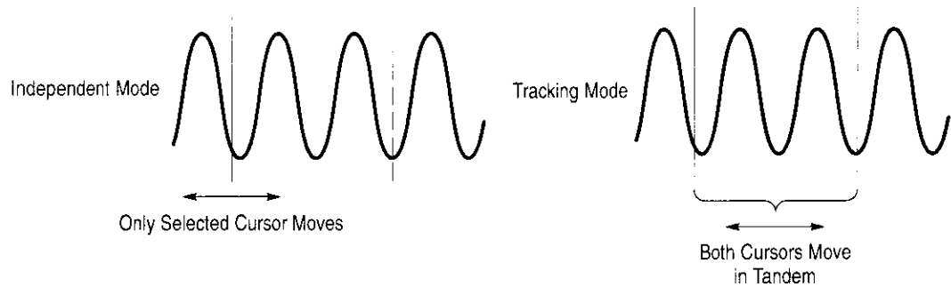
Figure 3-66: Cursor Modes
