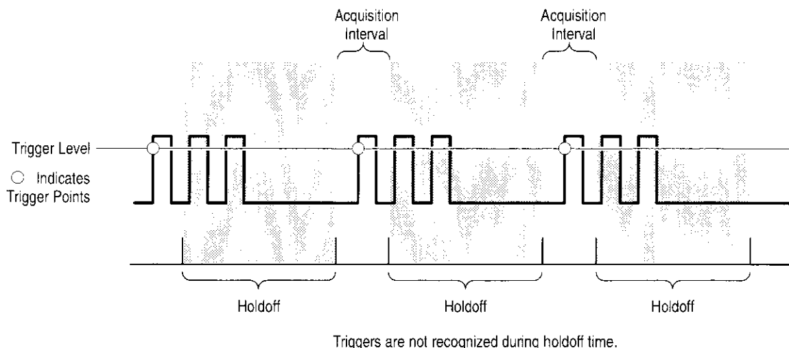
Figure 3–37: Trigger Holdoff Time Ensures Valid Triggering
