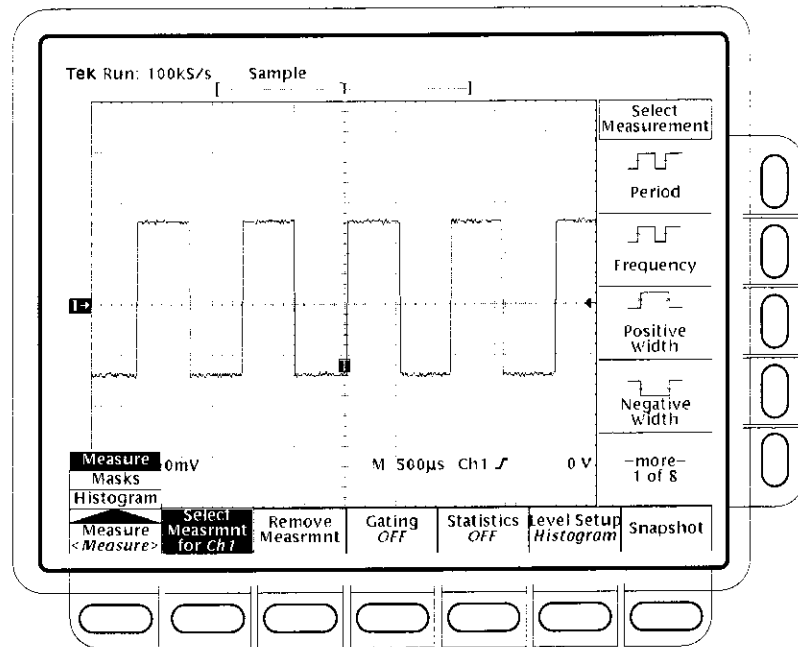
Figure 3–60: Measure Menu
