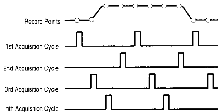
Figure 3–14: Equivalent-Time Sampling
