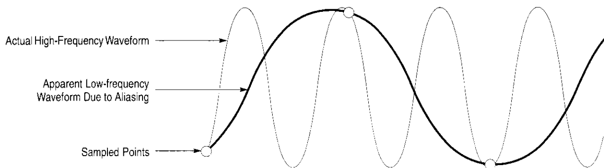
Figure 3–18: Aliasing
