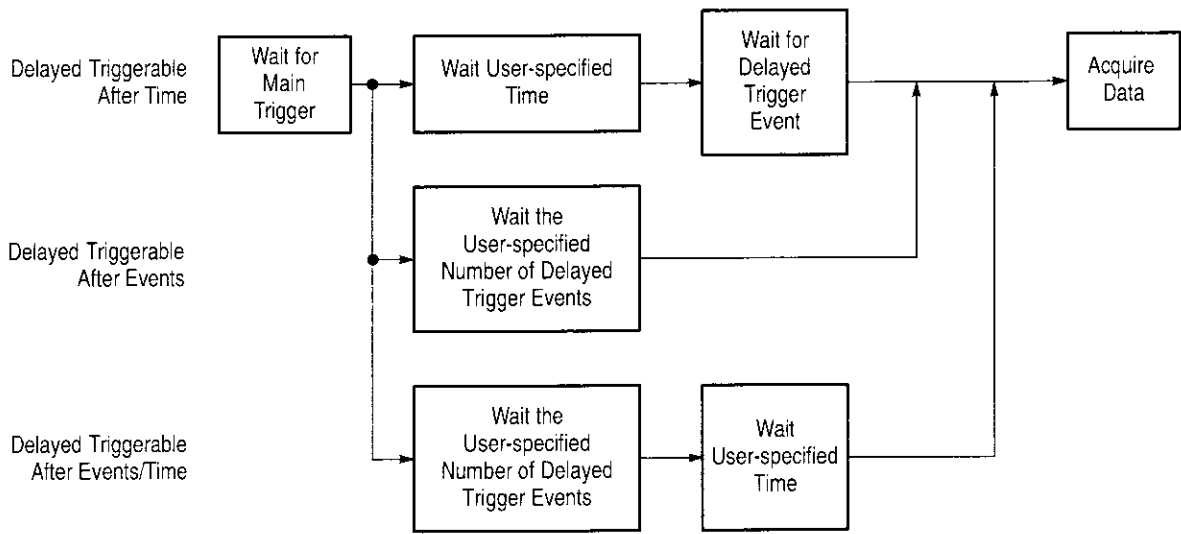
Figure 3–55: Delayed Triggerable
