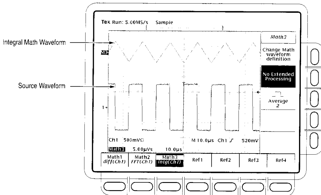
Figure 3-107: Integral Math Waveform
