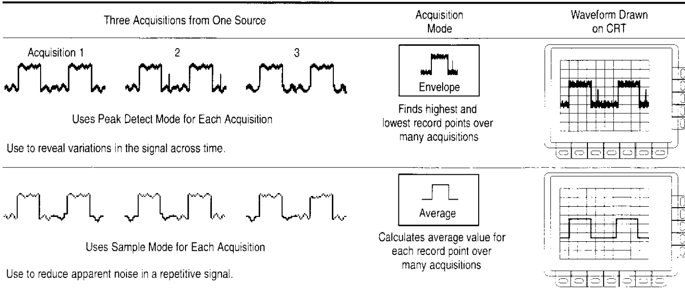
Figure 3-15: How the Acquisition Modes Work
