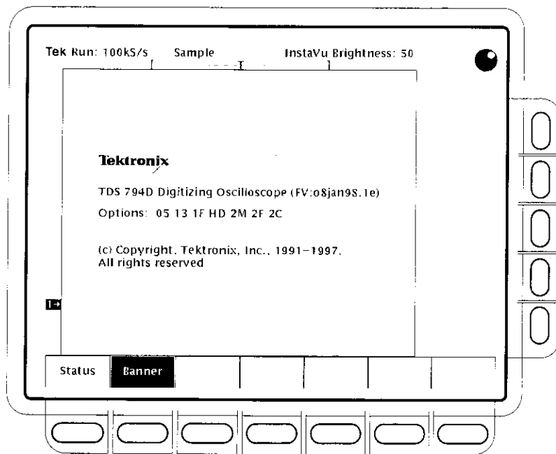
Figure 3–90: Banner Display
