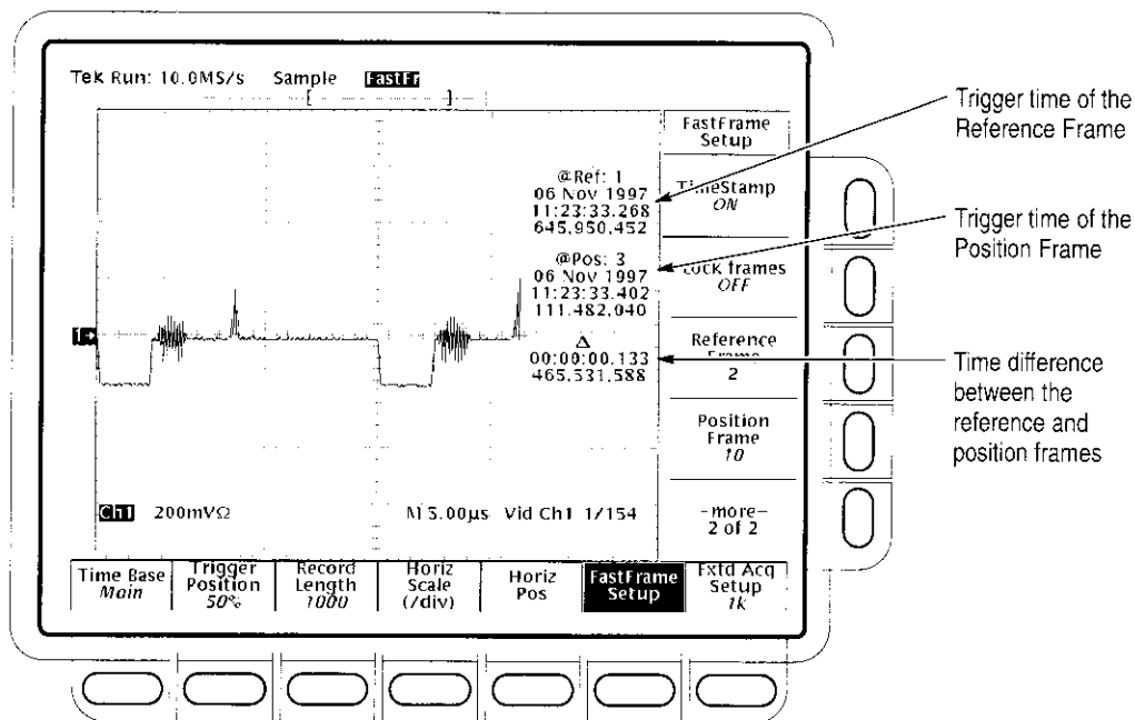
Figure 3-35: FastFrame TimeStamp
