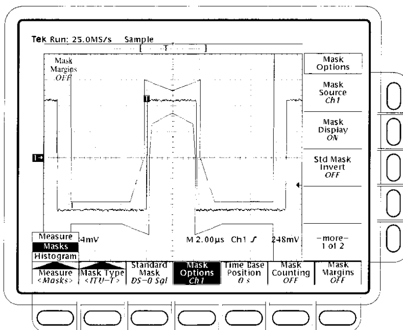
Figure 3–70: Mask menu
