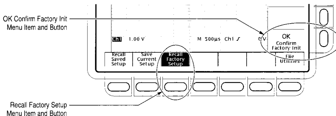
Figure 2-3: The Setup Menu
